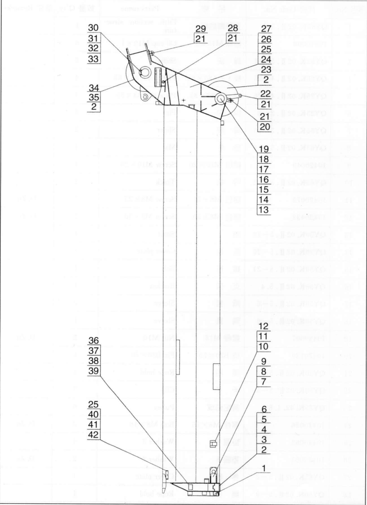
QY65K. 02 II. 5 五节臂 Fifth Section
