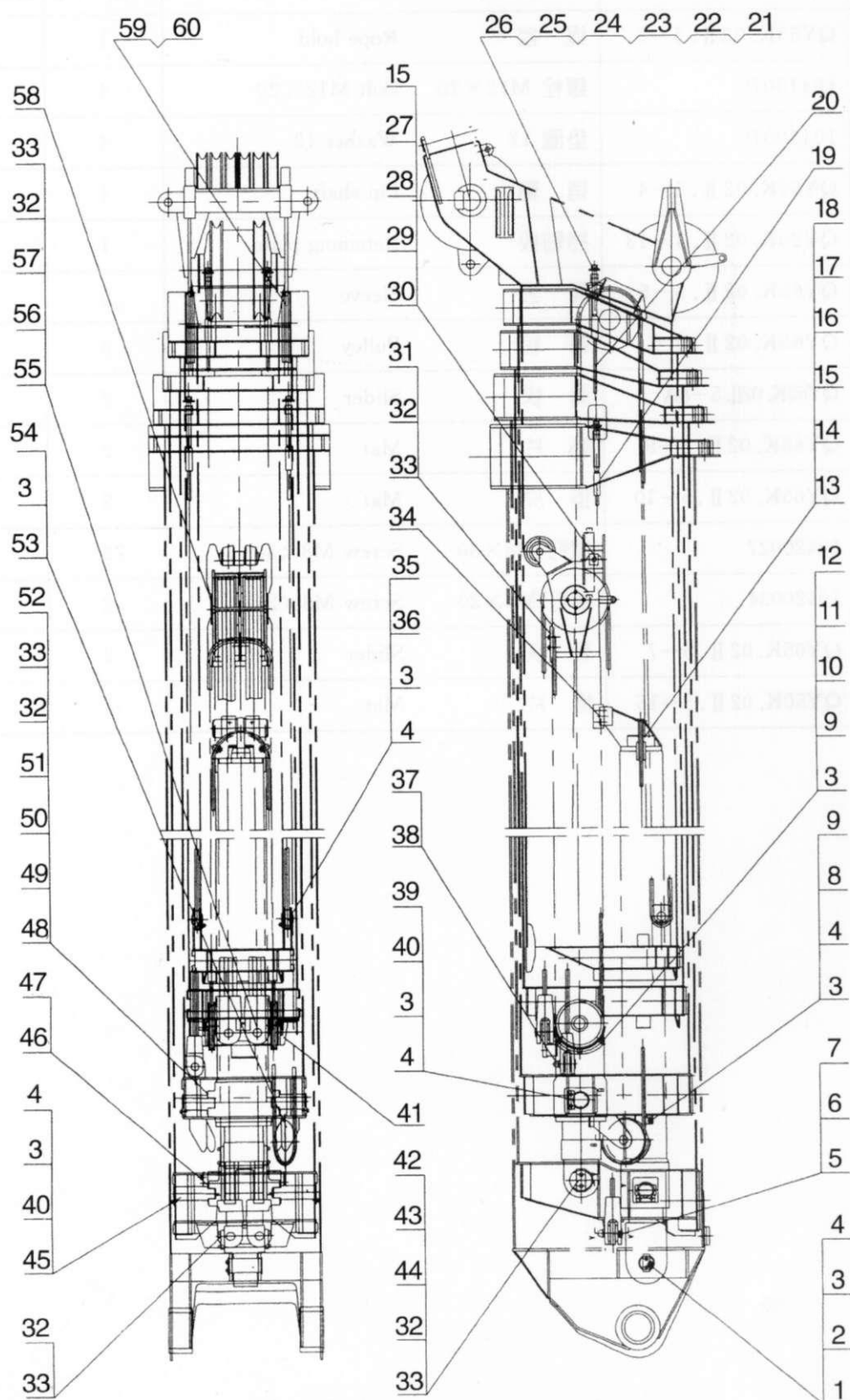
QY65K.02 II.6 伸缩机构 Telescoping Units
